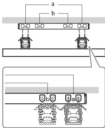
Hakens placering
